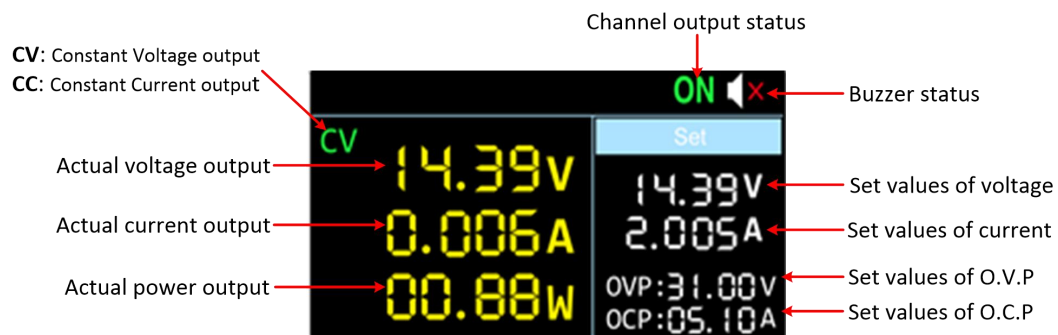
Figure 3- 3 User Interface
