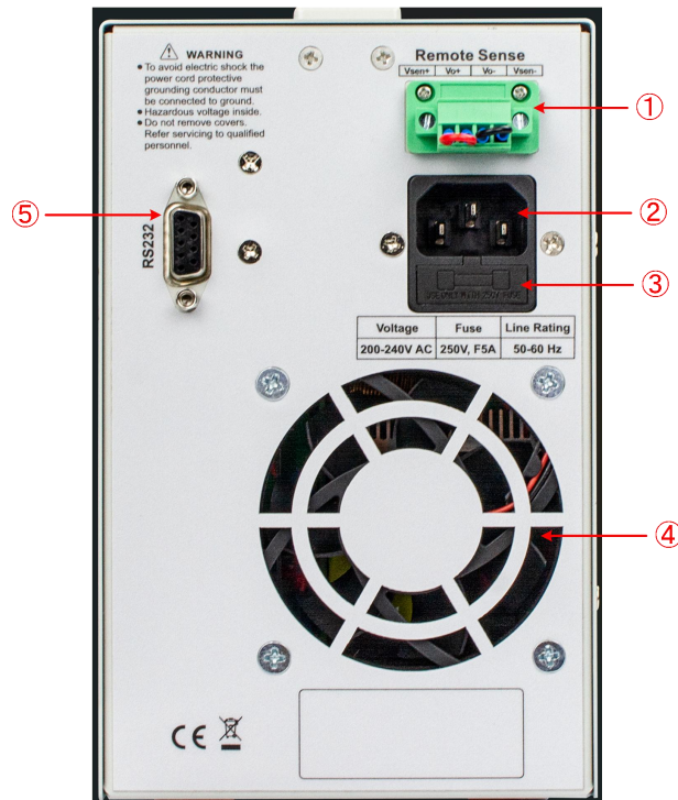
Figure 3- 3 80 Series Rear Panel Overview
