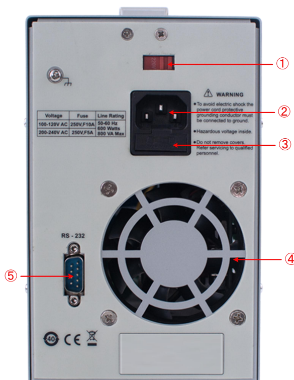
Figure 3- 2 Rear Panel Overview
