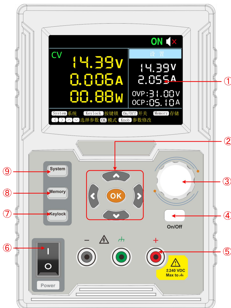
Figure 3-1 Front Panel Overview
